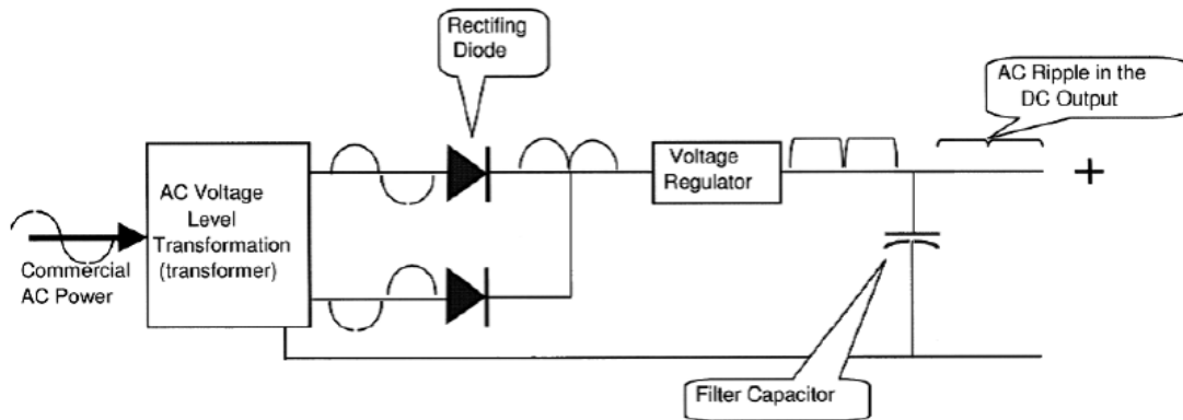
Figure 3: Rectification of AC voltage producing AC ripple
