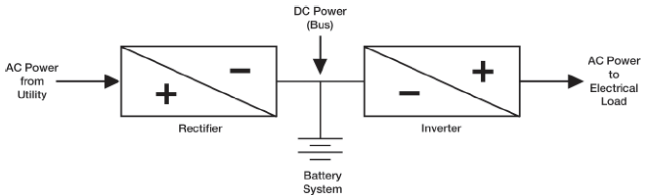
Figure 1: Typical UPS topology
