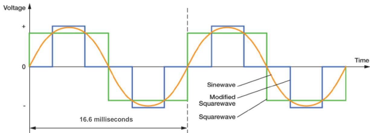
Figure 2: Inverter Output Sine wave
