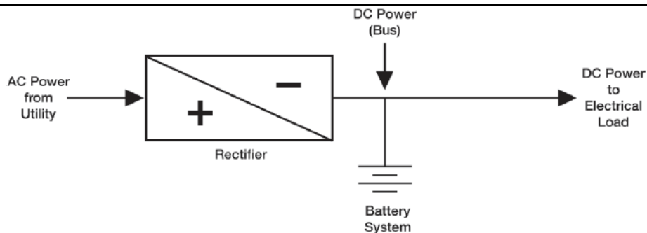
Figure 4: Typical DC Power System
